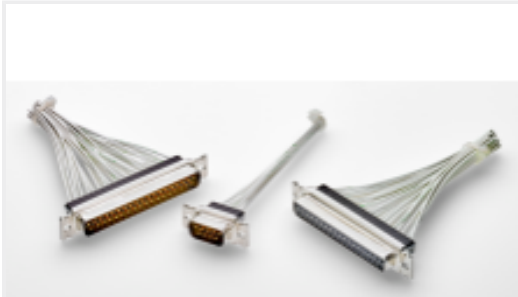
TE Part #2335893-1 AMPLIMITE SZ 1 RECPT 15 POS, ST STL SHEL
