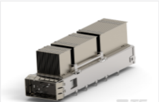
TE Part #2342934-3 QSFP-DD 1X1, STANDARD, W/ ZIPPER HS
