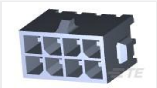
TE Part #3-794631-8 08P MICRO MNL ASSY,VRT,HDR LF
