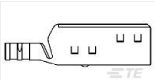
TE Part #520461-1 4 SDL RND SHIELD,BTTM,BULK PKG
