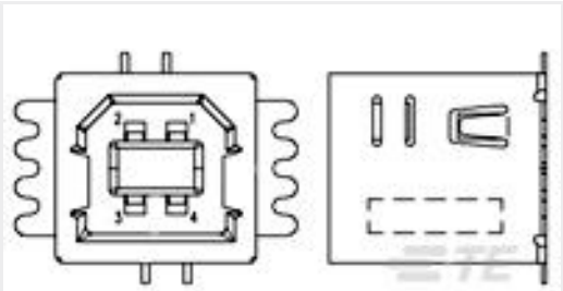
TE Part #1734517-1 STD USB TYPE B, VERTICAL, SMT, GRD FINGER
