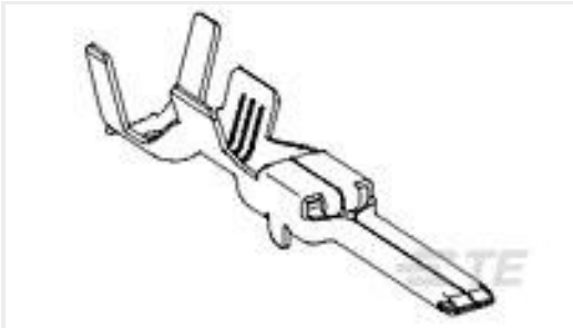
TE Part #1326031-5 2.8MM BLD,SEAL,14AWG
