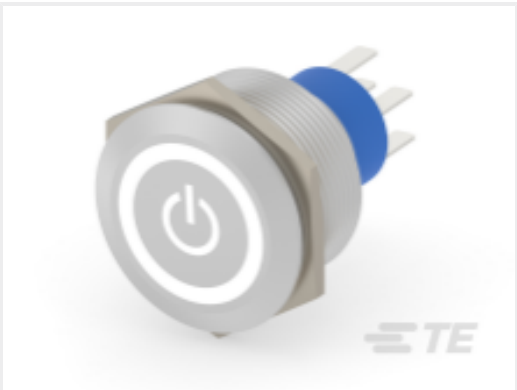
TE Part #2-2317658-6 AV25 DPL 3A MOVING RING POWER WHITE 24V
