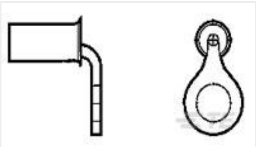
TE Part #322905 TERMINAL,SOLIS R 90DEG 1/0 1/4
