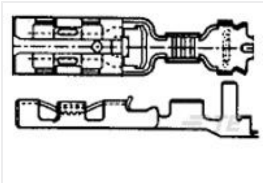
TE Part #353249-2 110 PL EX REC. 26-22AWG PTPHBZ
