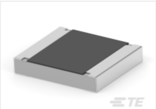
TE Part #3-2176346-4 CRGCQ 1210 330K 5%
