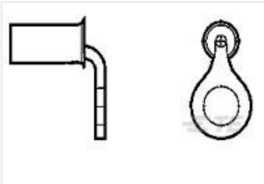
TE Part #35277 TERMINAL,SOLIS R 90DEG 8 1/4
