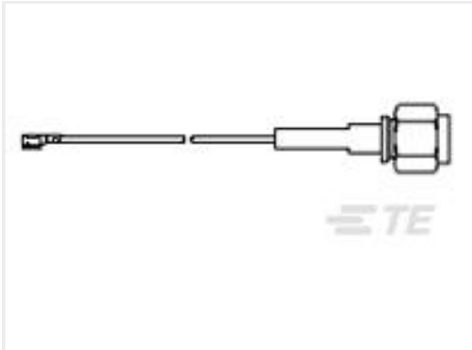
TE Part #2032439-1 RF CA,UMCC1 TO SMA PLUG,1.37 MM,L200MM
