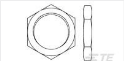
TE Part #1604196-1 NUT,JAM,5/8-24,PKG QTY 100
