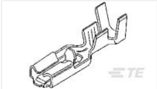
TE Part #63239-1 POSITIVE LOCK 250 REC 12-10 AWG TPBR
