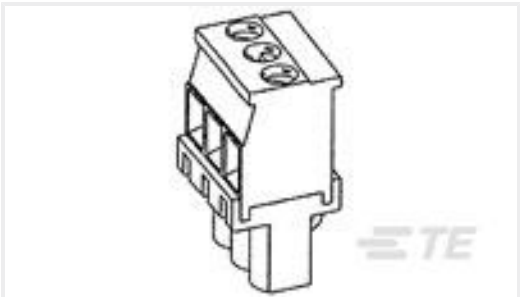
TE Part #1546105-5 5 POS 5.08MM LH PLUG BLCK
