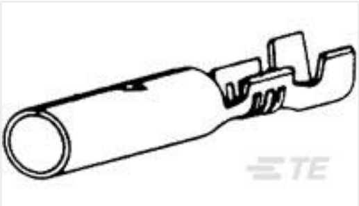
TE Part #60799-4 SHUR PLUG 180 REC 18-14 AWG TNPPHBZ
