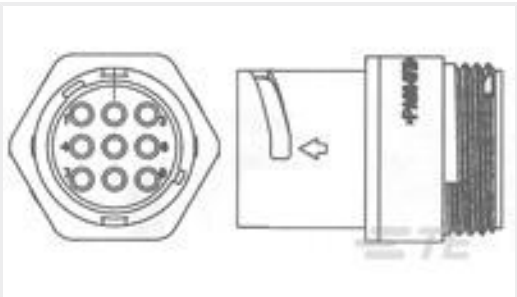
TE Part #1445828-3 REC,11-6,FRE HNG,LG INS,STD KE
