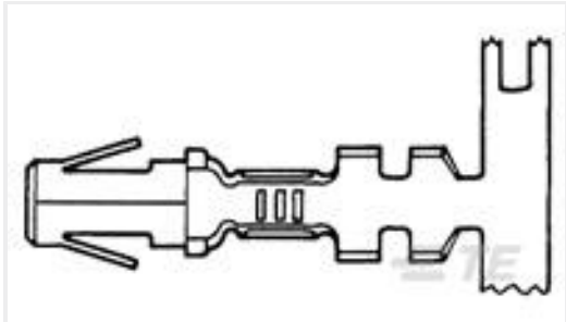
TE Part #350390-1 .140 DIA SOK 14-10 PTPBR L/P
