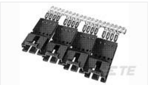
TE Part #5-103945-5 2X6 MTE SHRD PIN SR LATCH .100
