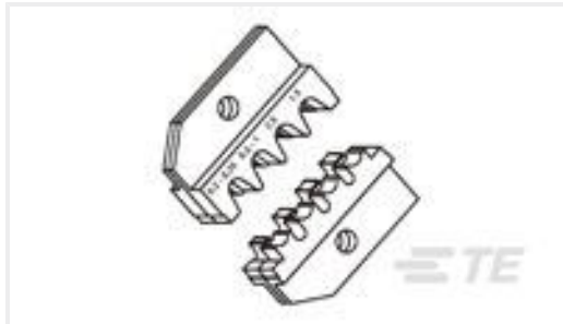
TE Part #4-1579001-6 ERGO DIE MCP 1,2 LL EDS
