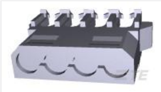
TE Part #794036-2 4P CMNL IDC PLUG 20AWG YEL V0
