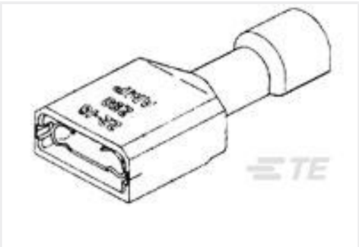
TE Part #3-520140-4 ULTRA-FAST 250 ASY REC 16-14 AWG TPBR
