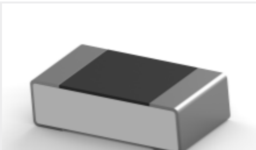
TE Part #5-2176370-7 RQ 0603 1K65 0.1% 10PPM 5K RL
