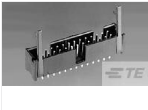
TE Part #104130-2 014 LOPRO HDR RA 30DP LATCH
