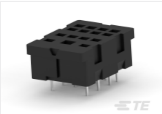
TE Part #3-1415043-1 PT78604
