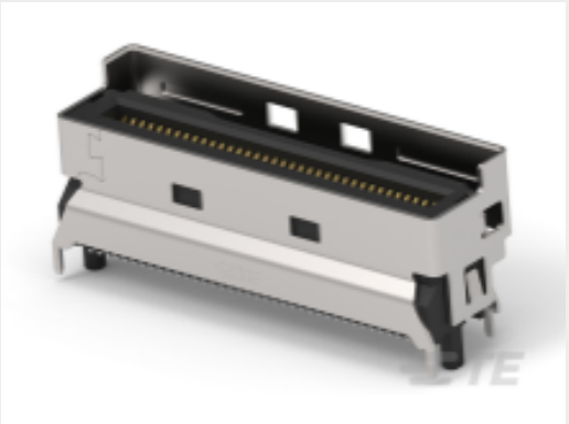
TE Part #1-2359366-5 MCIO INTERGRATED CONN, V/T,8X, SMT TYPE
