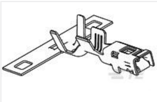
TE Part #1-1326032-1 2.8MM RECP,SEAL,14AWG,REV REEL
