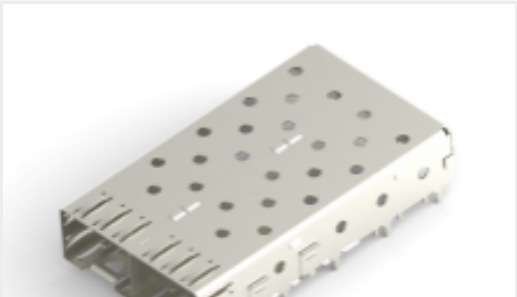
TE Part #1761014-3 SFP 1X2 CAGE ASSY, PRESS FIT
