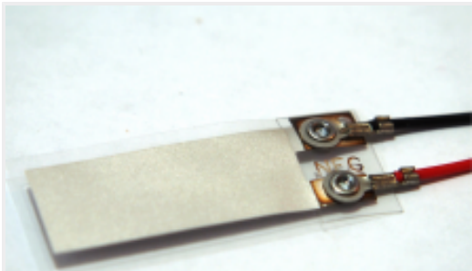
TE Part #11029075-00 LDT4-028K W/TH LEADS/RIVE
