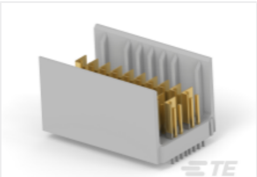
TE Part #2170328-1 HMZD+,2PAIRS,10COLS,VERTICAL, ASSEMBLY
