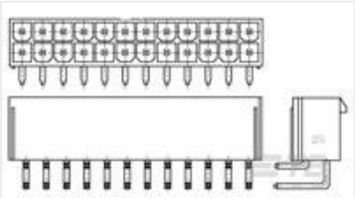
TE Part #1-1586041-6 16P VAL-U-LOK R/A HDR V2
