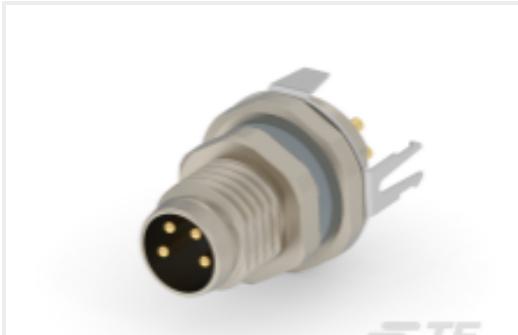
TE Part #T4040034041-000 M8.MLE.PNLREAR.4POS.STR PCBSHLD
