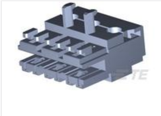
TE Part #1534415-3 DUOPL POW FEM CON3P
