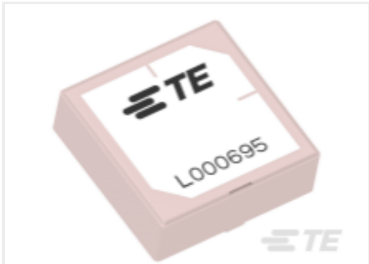
TE Part #L000695-01 Ceramic Patch ant, 1561-1602MHz, 18x18x6
