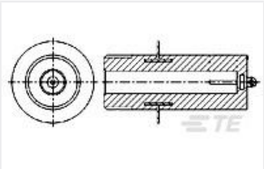
TE Part #861257-1 RECEPTACLE
