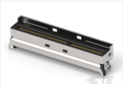
TE Part #1-2381578-7 MCIO INTERGRATED CONN, V/T, 124P SMT TYPE
