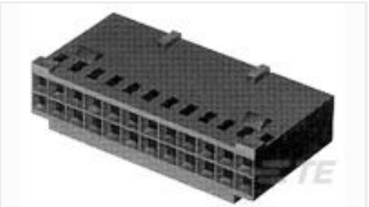
TE Part #87631-7 12 MODIV HSG COMP DR .100 POL
