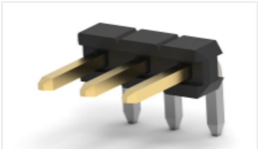
TE Part #2842110-3 3P,2MM,BRK HDR,SRRT,2.8,0.1AU,TB
