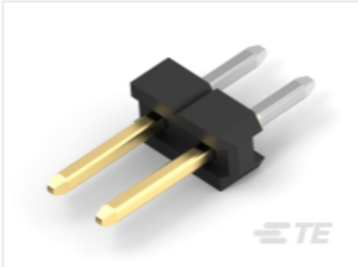
TE Part #2355182-2 2P,2MM,BRK HDR,SRVT,2.8,0.76AU,TB
