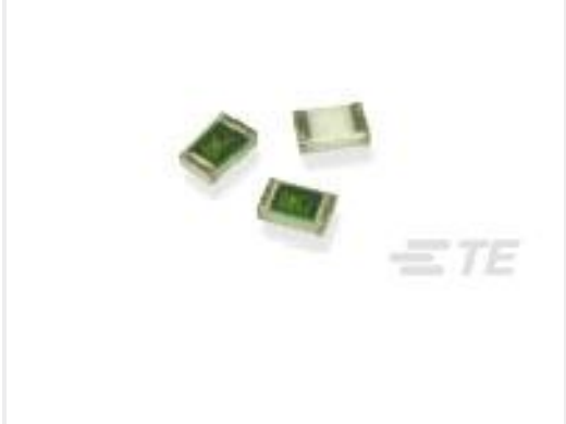
TE Part #8-1625867-1 RP 1J 0.166W 43R2 0.1% 25PPM 1K RL
