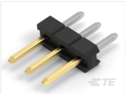
TE Part # 2355045-3 3P, 2MM, BRK HDR, SRVT, 2.8, 0.1AU, TB
