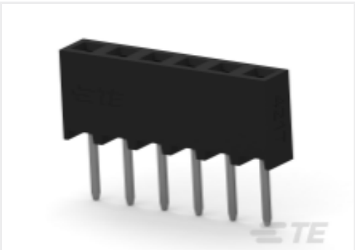
TE Part #2314878-6 6P,2MM,B-B,REC,SRVT,2.7,0.76AU,TB
