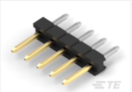
TE Part # 2355186-5 5P,2MM,BRK HDR,SRVT,2.8,0.76AU, BOX
