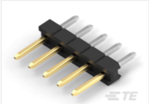
TE Part # 2355184-5 5P,2MM,BRK HDR,SRVT,2.8,0.76AU,TB W/CAP
