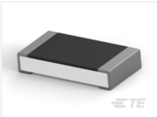
TE Part #4-2176388-0 RQ 1206 25R5 0.1% 10PPM 5K RL
