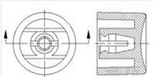
TE Part #1825068-2 C22204 CAP RED
