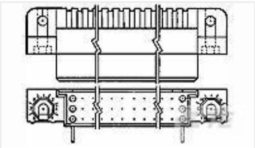
TE Part #533914-2 HDI RECP ASSY 3 ROW 96 POS
