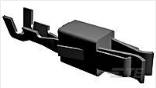
TE Part #927774-3 JPT REC 2.8 Contact SRC Sn
