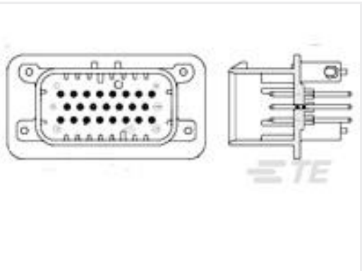
TE Part #776200-1 23POS,PIN DIA 1.3,HDR ASSY, 180DEG,COD 1
