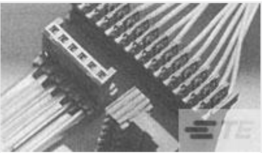
TE Part # 281708-3 PLUG HE14 IDC 90 3 P TUBE
