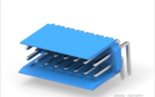
TE Part #CAT-AM74-H3401C HE13/HE14 TH Headers, DRRA
