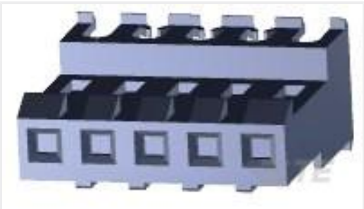
TE Part #3-640600-5 05P MTA156 CONN ASSY 20AWG LF
