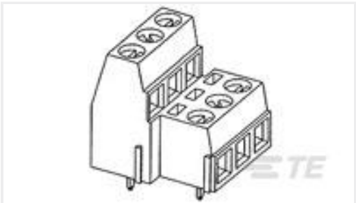
TE Part #796692-3 TERMI-BLOK PCB MOUNT 1&2 3P.5
