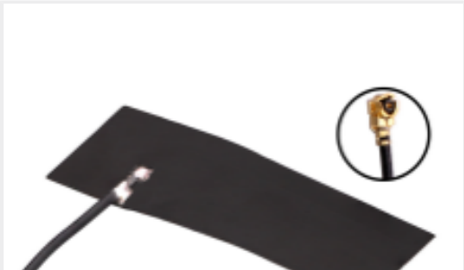
TE Part #L9000126-01 Antenna FPC Sub-6 LTE/5G 1.13 100 UFL
