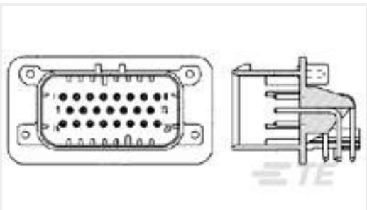
TE Part #776267-1 14POS,PIN DIA 1.3,HDR ASSY,90DEG, COD 1
